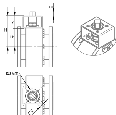
B1322FA with ISO 5211 bracket
